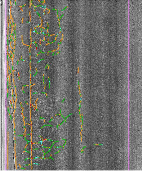
Figure 3: Example of crack map overlaid on 3D image
