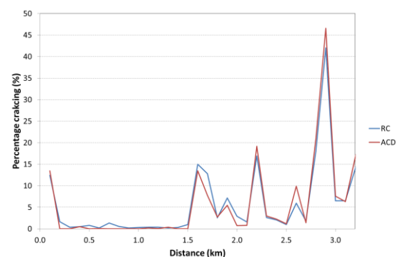
Figure 6: Comparison of ACD and RoadCrack outputs on dense graded asphalt
