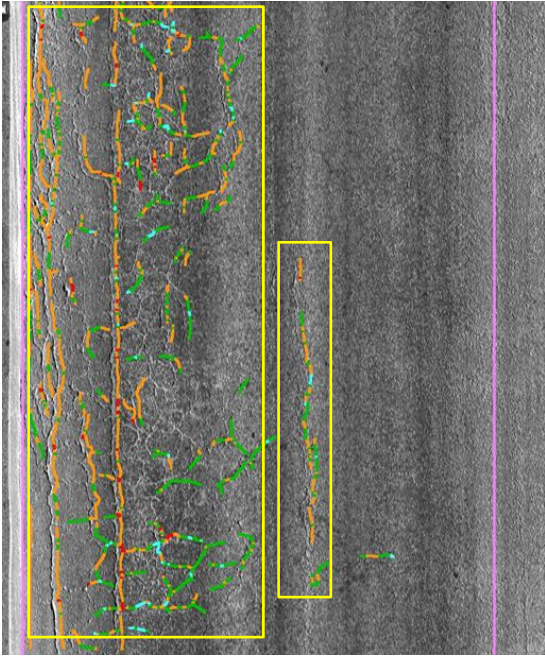
Figure 4: Example of crack type identification
