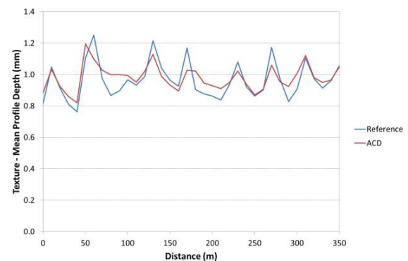
Figure 11: Texture comparison between ACD and reference device
