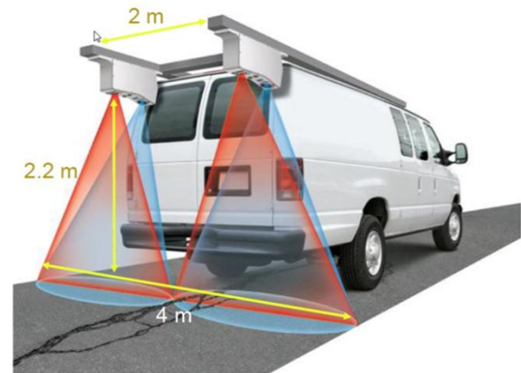
Figure 2: Configuration and measurement range of ACD (picture courtesy of Pavemetrics)
