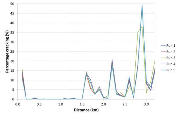
Figure 5: ACD repeatability on dense graded asphalt
